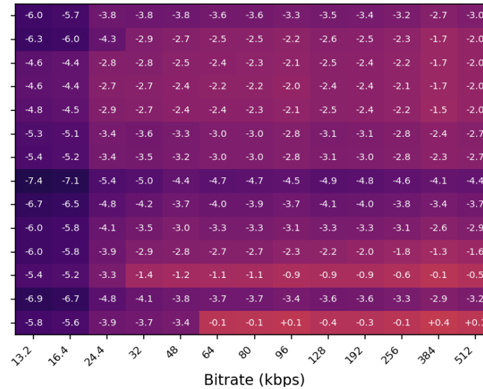
Output Loudness Heatmap across Bitrates: ISM4MASA1DIR1 SWB | ref -14.0 LKFS
