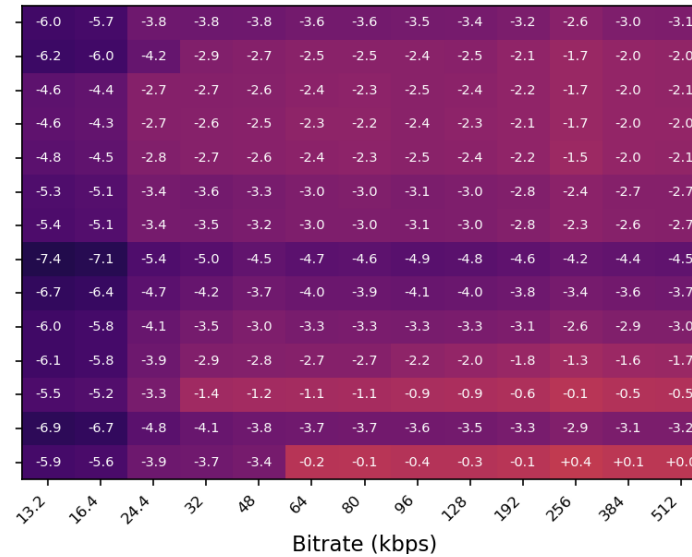
Output Loudness Heatmap across Bitrates: ISM3MASA1DIR1 SWB | ref -14.0 LKFS
