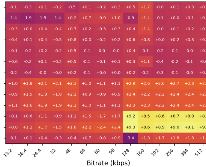
Output Loudness Heatmap across Bitrates: 7_1_4 SWB | ref -19.5 LKFS
