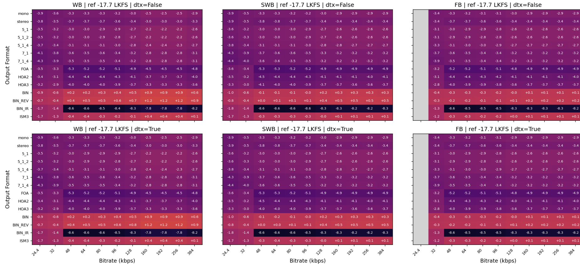
Output Loudness Heatmap across Bitrates: ISM3
