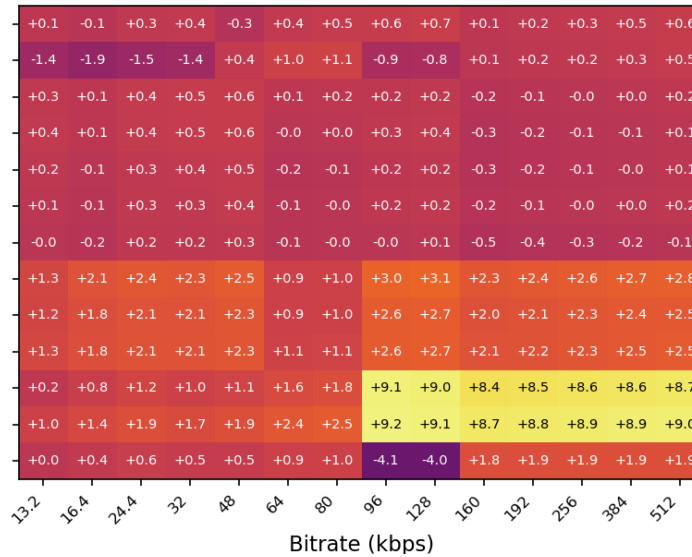
Output Loudness Heatmap across Bitrates: 5_1_4 SWB | ref -20.0 LKFS
