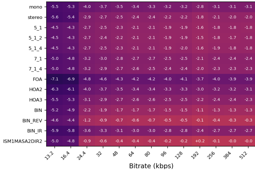
WB | ref -15.8 LKFS
