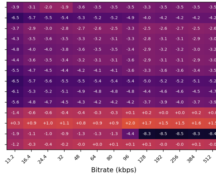
Output Loudness Heatmap across Bitrates: ISM2SBA2 SWB | ref -16.9 LKFS
