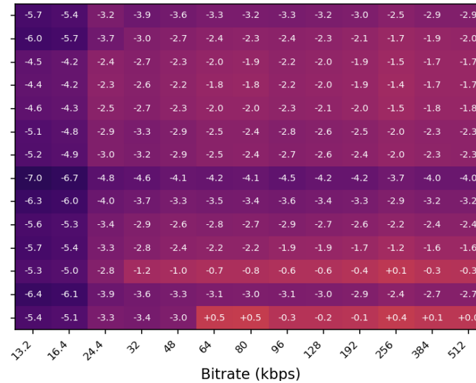
Output Loudness Heatmap across Bitrates: ISM3MASA2DIR2 SWB | ref -14.7 LKFS
