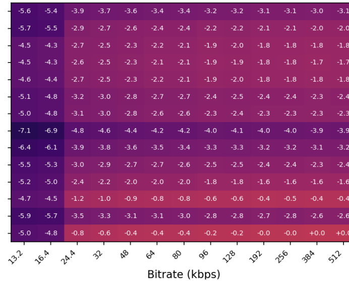
Output Loudness Heatmap across Bitrates: ISM1MASA2DIR2 SWB | ref -15.8 LKFS
