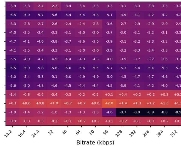
Output Loudness Heatmap across Bitrates: ISM3SBA3 SWB | ref -15.7 LKFS
