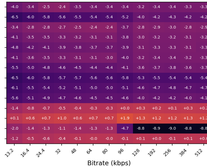
Output Loudness Heatmap across Bitrates: ISM3SBA2 SWB | ref -15.7 LKFS
